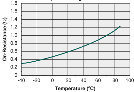
Typical On-Resistance vs. Temperature ( I_F=20\text{mA} , I_L=0.75\text{A} )
