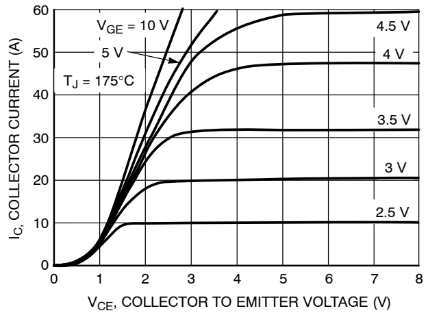
Figure 4. Collector Current vs. Collector-to-Emitter Voltage
