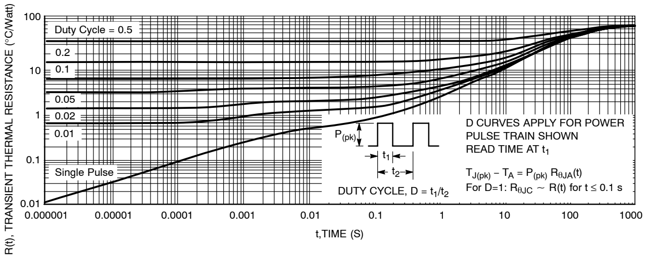
Figure 13. Minimum Pad Transient Thermal Resistance (Non-normalized Junction-to-Ambient)
