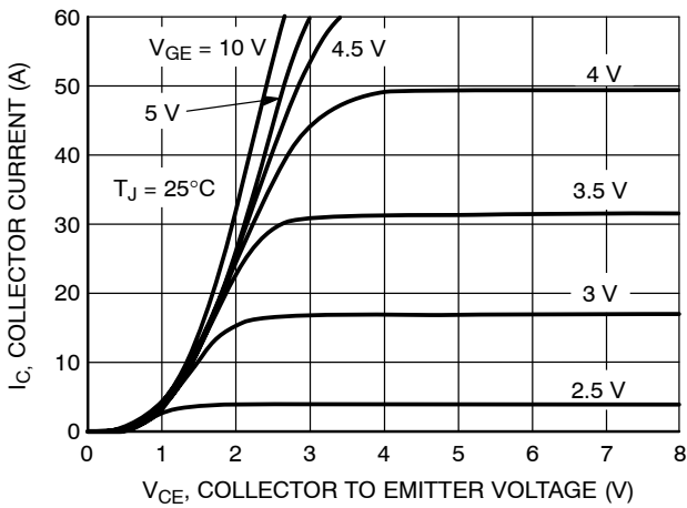
Figure 5. Collector Current vs. Collector-to-Emitter Voltage
