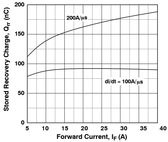
Figure 21. Stored Charge
